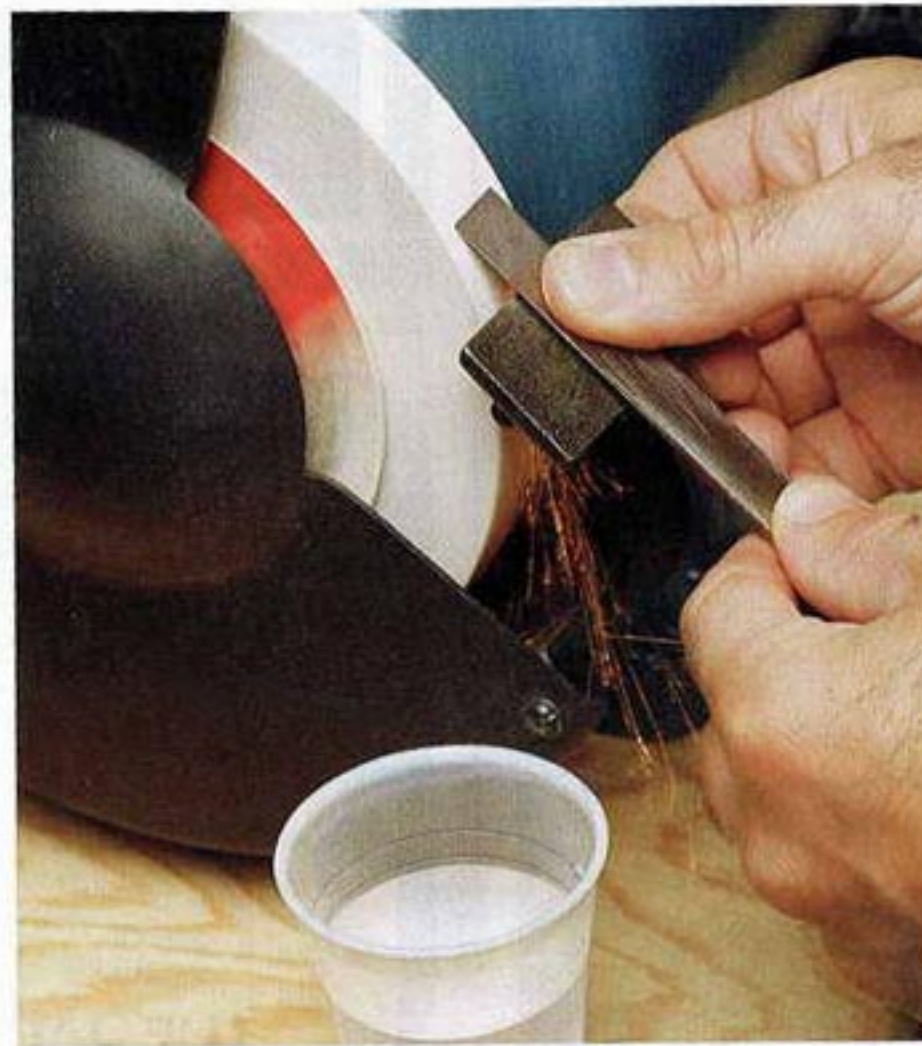
The key to grinding metal is to keep it from overheating. Use a light touch and pause often to dunk the tool in water. Aluminum-oxide wheels, usually white or pink, produce less heat than standard-grit gray Carborundum wheels. Slow-speed motors also help.
