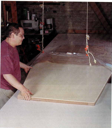
It doesn't take a lot of pressure. The honeycomb core requires only about half of the clamping pressure as that used for gluing up veneer.
