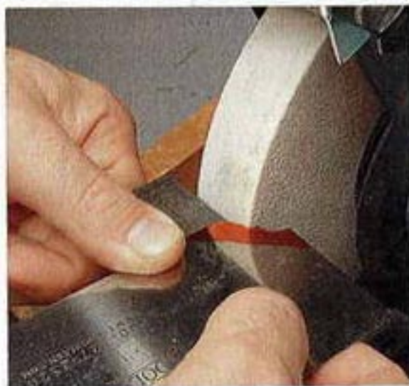
Grind close to the line. Set the tool rest perpendicular to the grinding wheel, and use the corner of the wheel to reach into concave areas of the profile.
