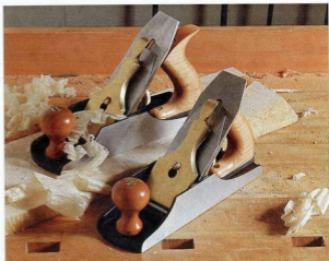
The lowdown on a high frog. The high-angled (50°) frog (on the plane in back) cuts at a steeper angle than a typical 45° frog (front). A steep angle is less likely to cause tearout when planing uneven grain.
